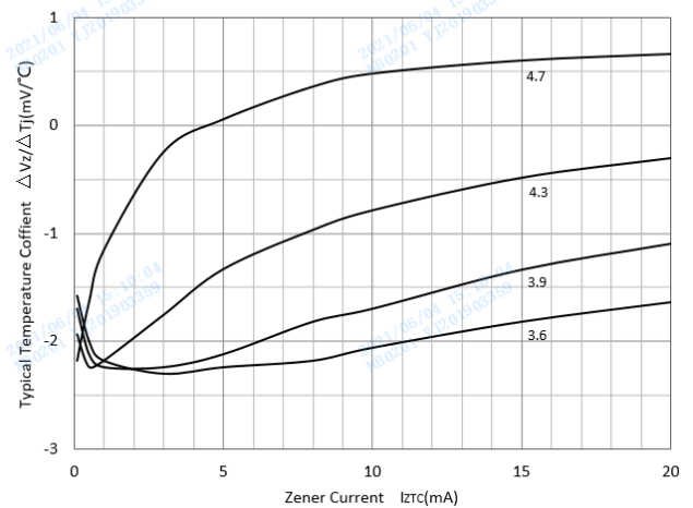
Temperature coefficient
